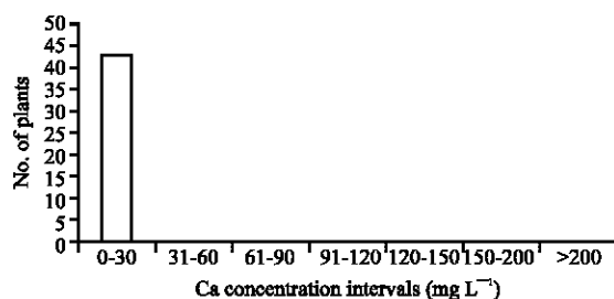
Fig. 9: Calcium Concentration intervals for desalinated water from small-scale BWDPs in Gaza Strip
