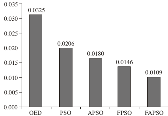
Fig. 15: Voltage deviation
