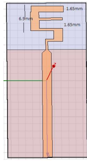
Figure 3: The E-shaped MLA antenna
